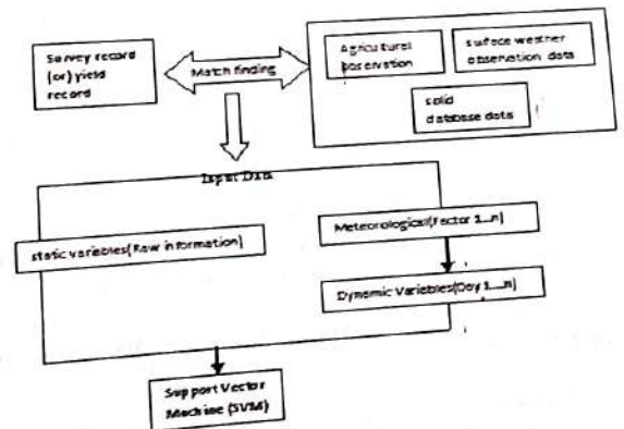
Figure 2. Flow chart SVM algorithm
